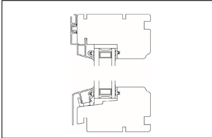
Figure 1 Typical vertical section of an FA Fixed Window
