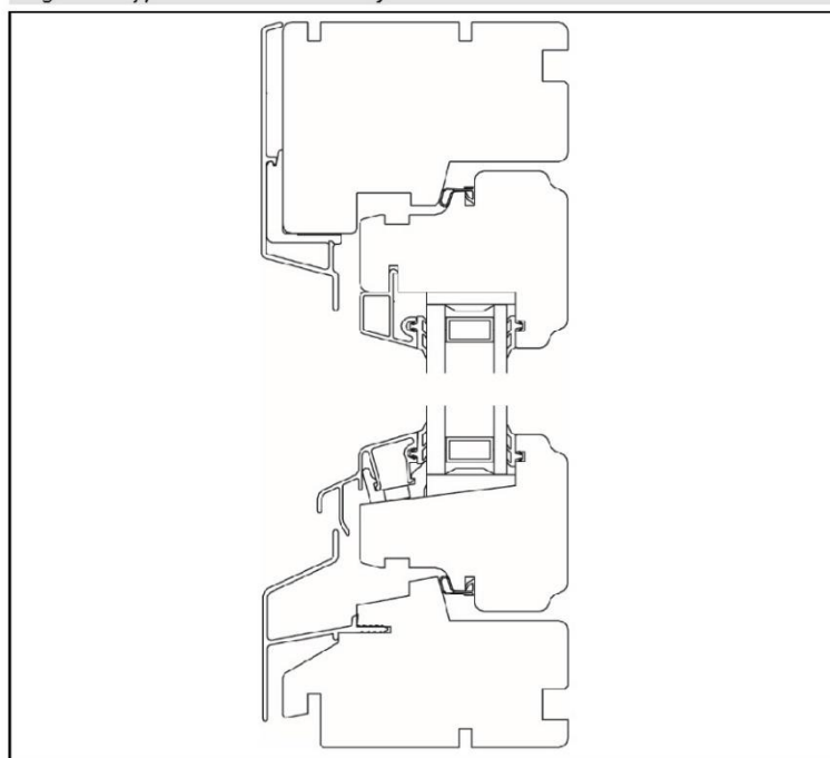
Figure 1 Typical vertical section of an ND 3-Handled Tilt and Turn Window
