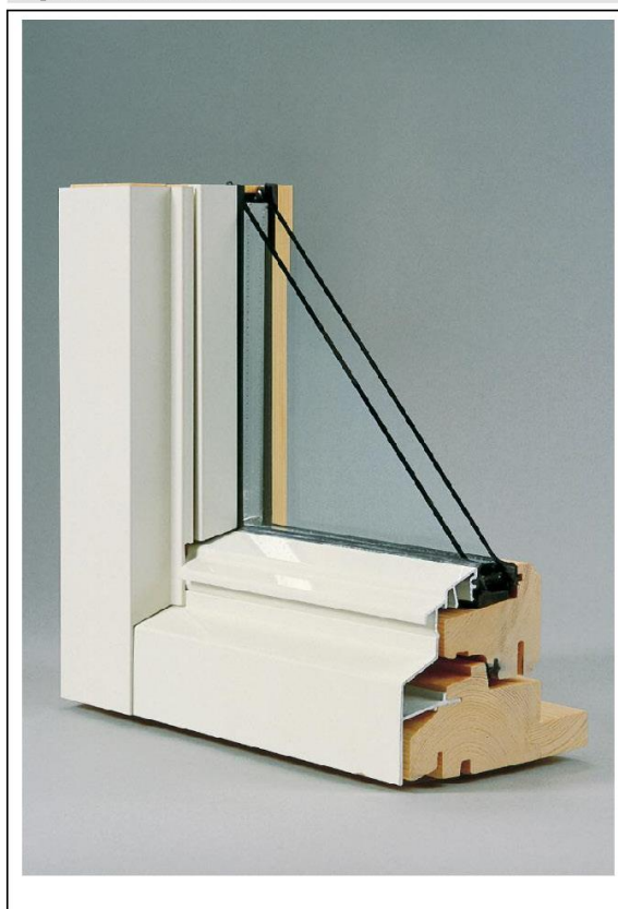
Figure 1 Corner detail
