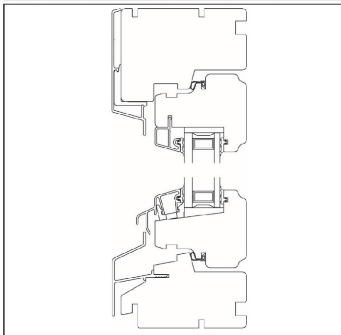
Figure 2 Typical vertical section (showing aluminium cladding)
