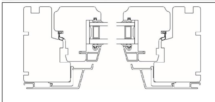
Figure 3 Typical horizontal section (showing aluminium cladding)
